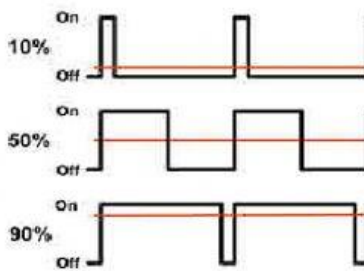
PULSE WIDTH MODULATION - PWM
