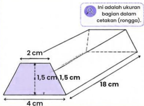
Diagram Prisma Trapesium
