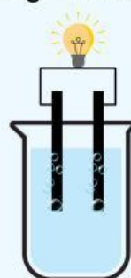
\text{NH}_3
