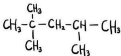
Gambar 2. isooktana
