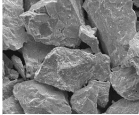
Gambar 4. Karbit ( \text{CaC}_2 )
