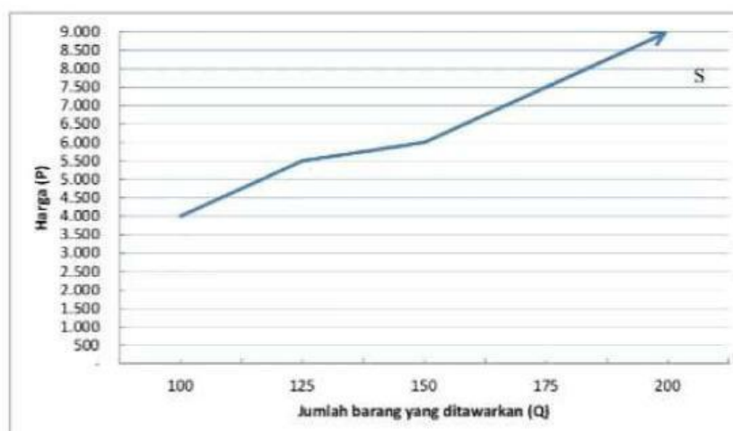
Gambar 2.2 Kurva Penawaran
