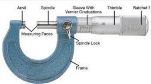
Micrometer
