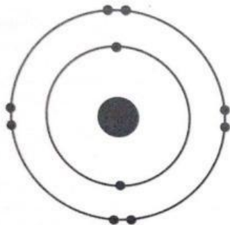
Atom stabil Stable atom
