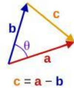
trigonometry
