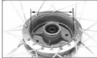
Gambar 5. 12 Mengukur Diameter Tromol
