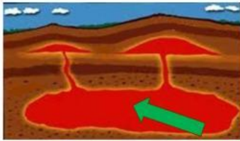
magma
