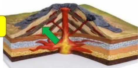
layers
