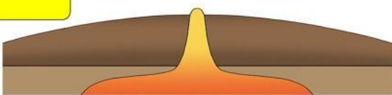
shield volcano
