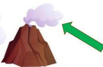
ash
