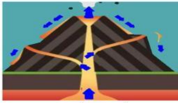
composite volcano
