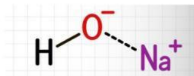
Gambar 4. Struktur molekul NaOH Sumber : https://www.istockphoto.com
