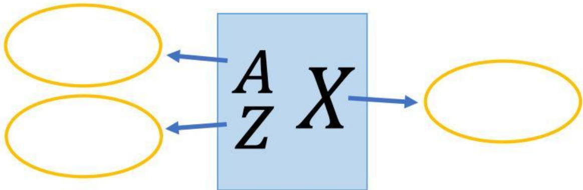
Gambar 1 – Lambang Atom
