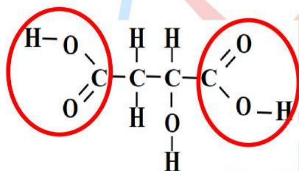
Malic acid
