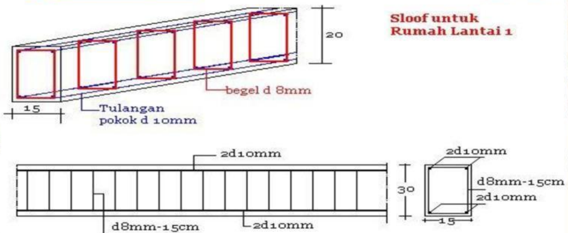
Gambar Sloof
