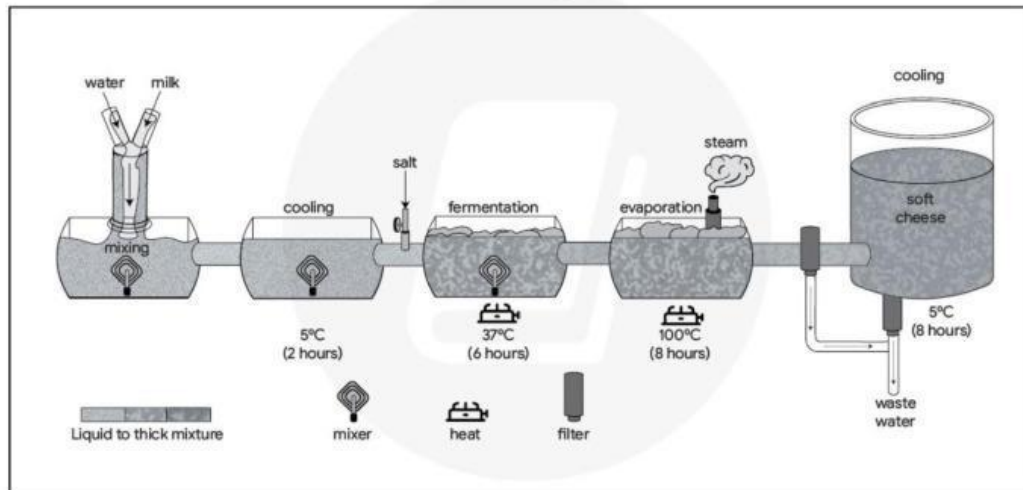
Process for making soft cheese
