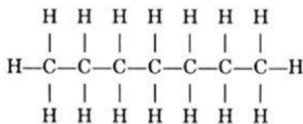
Gambar 3. n-heptana
