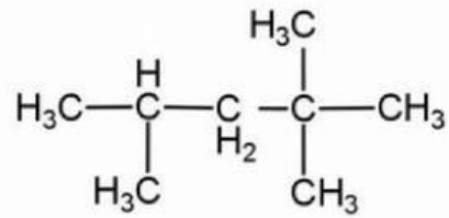
Gambar 2. Isooktana
