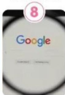
SEARCH ENGINE
