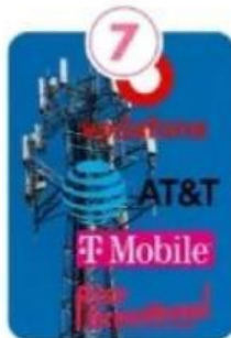
INTERNET PROVIDER
