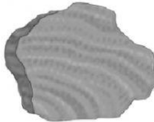
Sandstone
