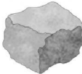
Granite
