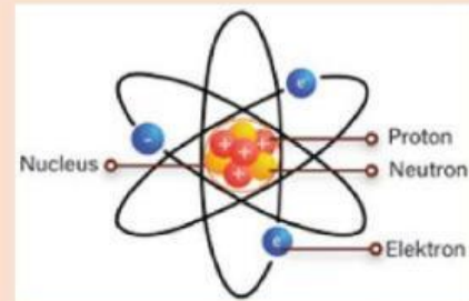
Gambar Atom Rutherford
