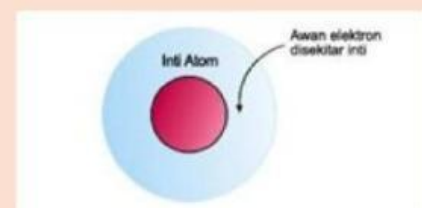
Gambar Atom Mekanika Kuantum
