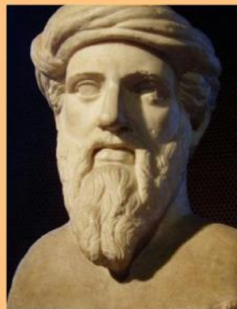
Pythagoras
