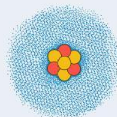
Mekanika Kuantum
