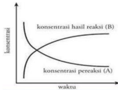
Gambar 2 Diagram Laju Reaksi
