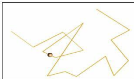
Gambar 5. Gerak Brown
