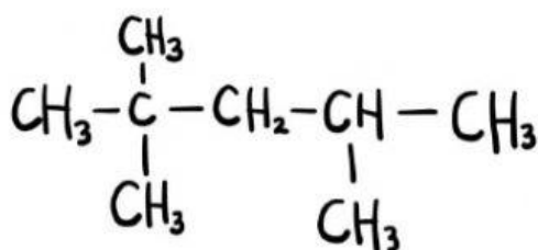
Gambar 2. isooktana
