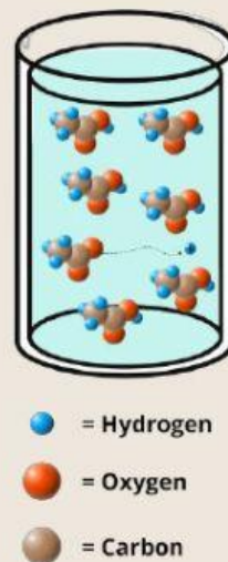
Gambar 1b. Larutan CH 3 COOH
