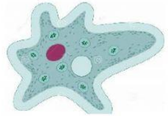
amoeba
