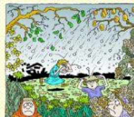
hail
