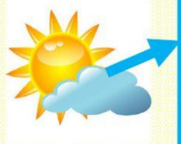
clearing up
