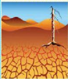
dry
