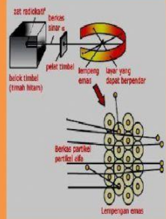
Percobaan Rutherford
