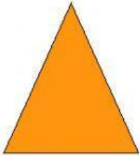
triangles
