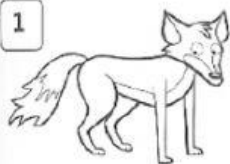
fox
