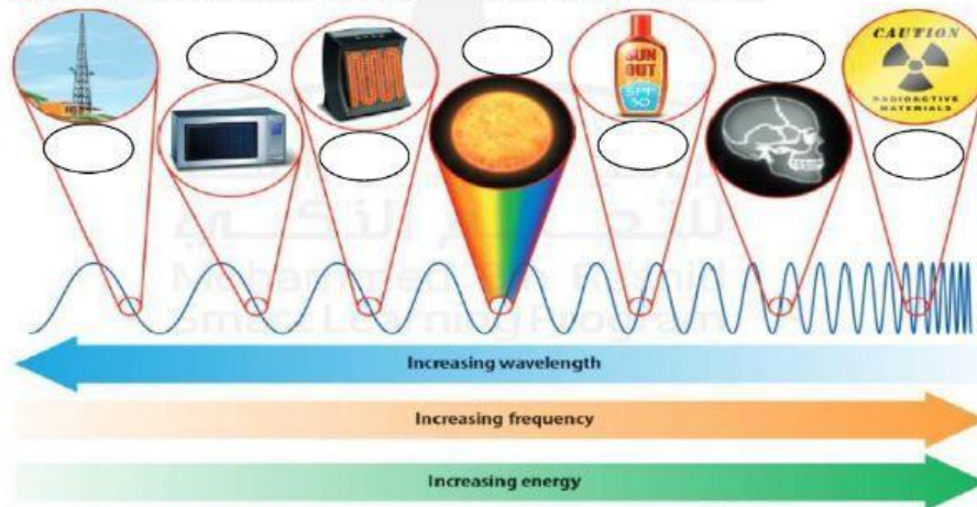
Figure 13 Electromagnetic waves have different wavelengths, frequencies, and energy.
