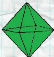
OCTAEDRO REGULAR
