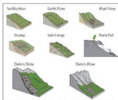
Figure 4.8 Mass Movement
