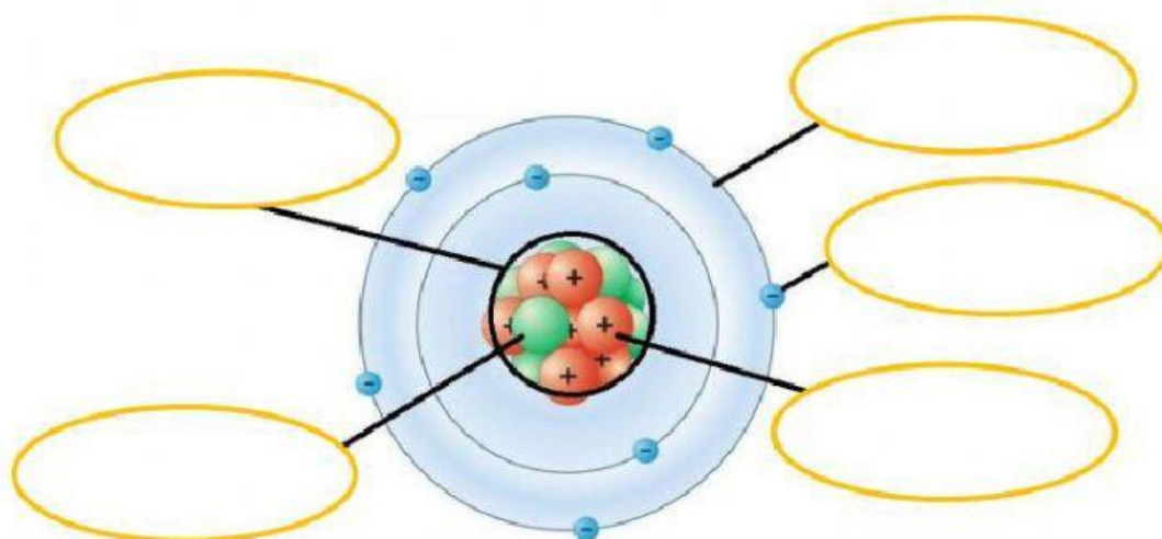
Gambar 2 - Bagian-bagian Atom
