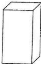
parallelepipedo
