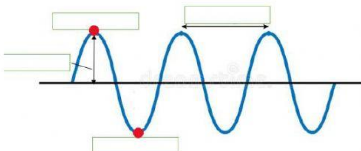
Transverse Wave
