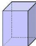
Prisma rectangular
