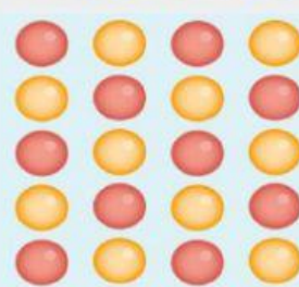
Homogeneous mixture
