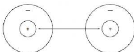
Figure 3.4: Repulsion between protons
