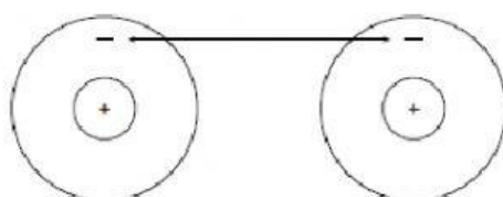
Figure 3.2: Repulsion between electrons
