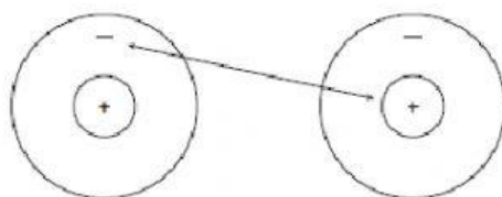
Figure 3.3: Attraction between electrons and protons.
