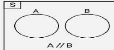
Diagram Venn Saling Lepas
