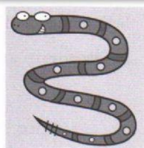
8. snake
