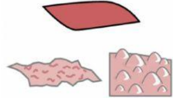
Texture
