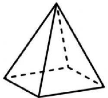
Square-based pyramid
