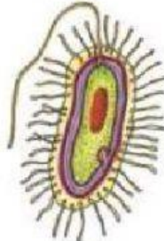
Bacteria
