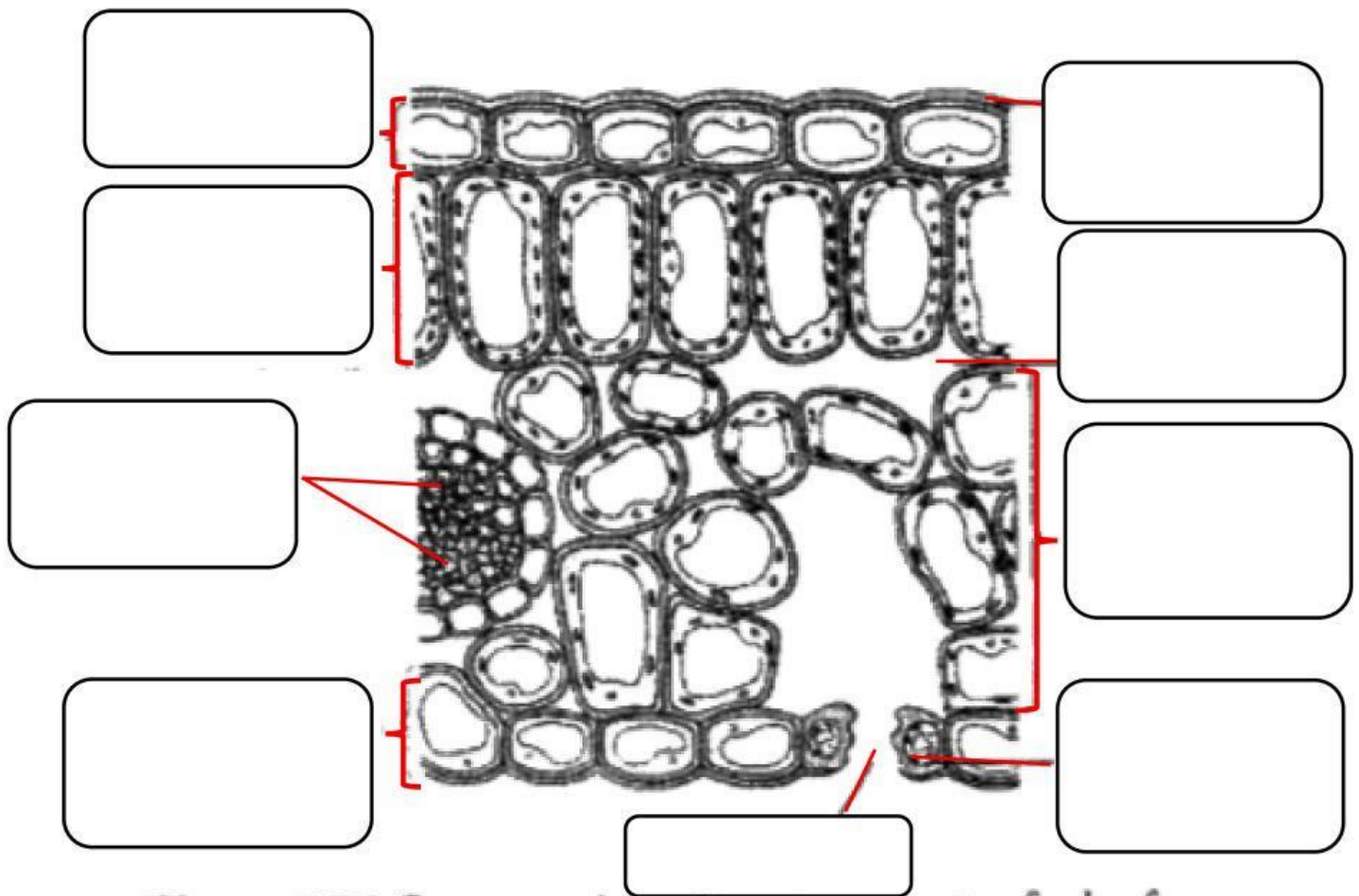
Figure 6.50 Cross-section of various parts of a leaf
