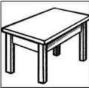
desk | dog
