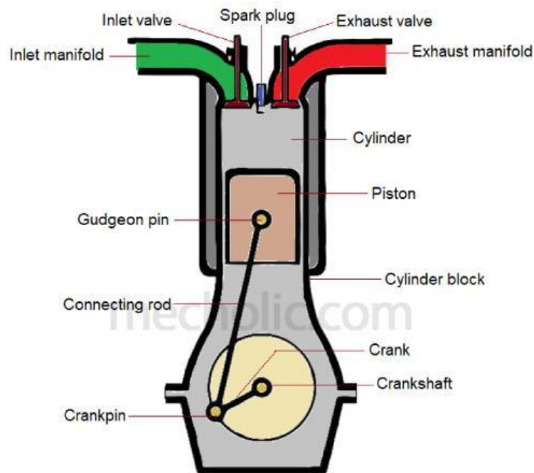
Basic components of IC Engine
