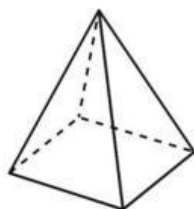
square-based pyramid
