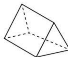
triangular prism
