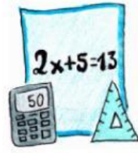
Equation
