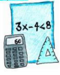
Inequation
